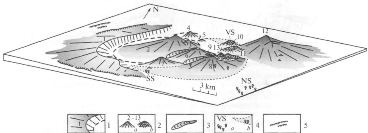
Fig. 2. A block diagram for the Bol'shoi Semyachik Volcanic Massif.
