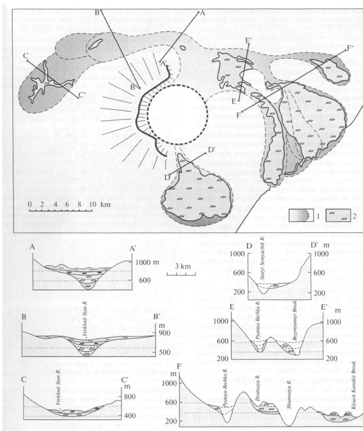
Fig. 5. A map showing the distribution of pyroclastic flows related to the generation of the Bol'shoi Semyachik caldera (top) and sections that cut across the trend of individual flows (bottom).
