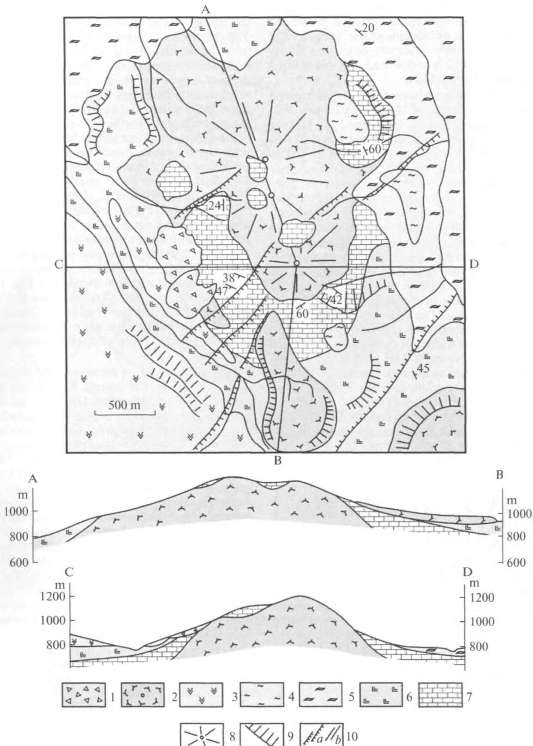
Fig. 7. Geological structure of the Kulakova dome.
