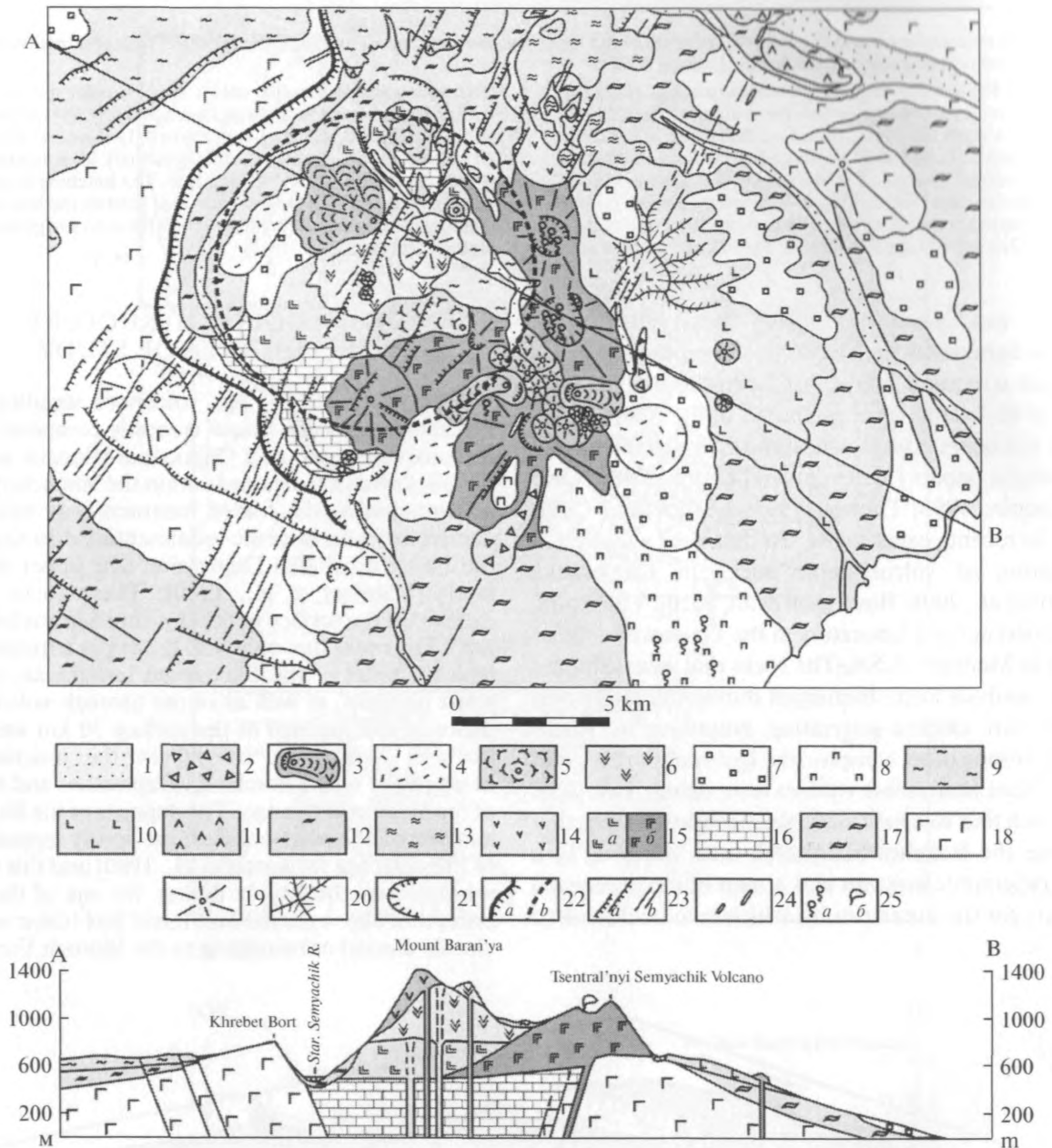
Fig. 3. A schematic geological map of the Bol'shoi Semyachik Volcanic Massif.
