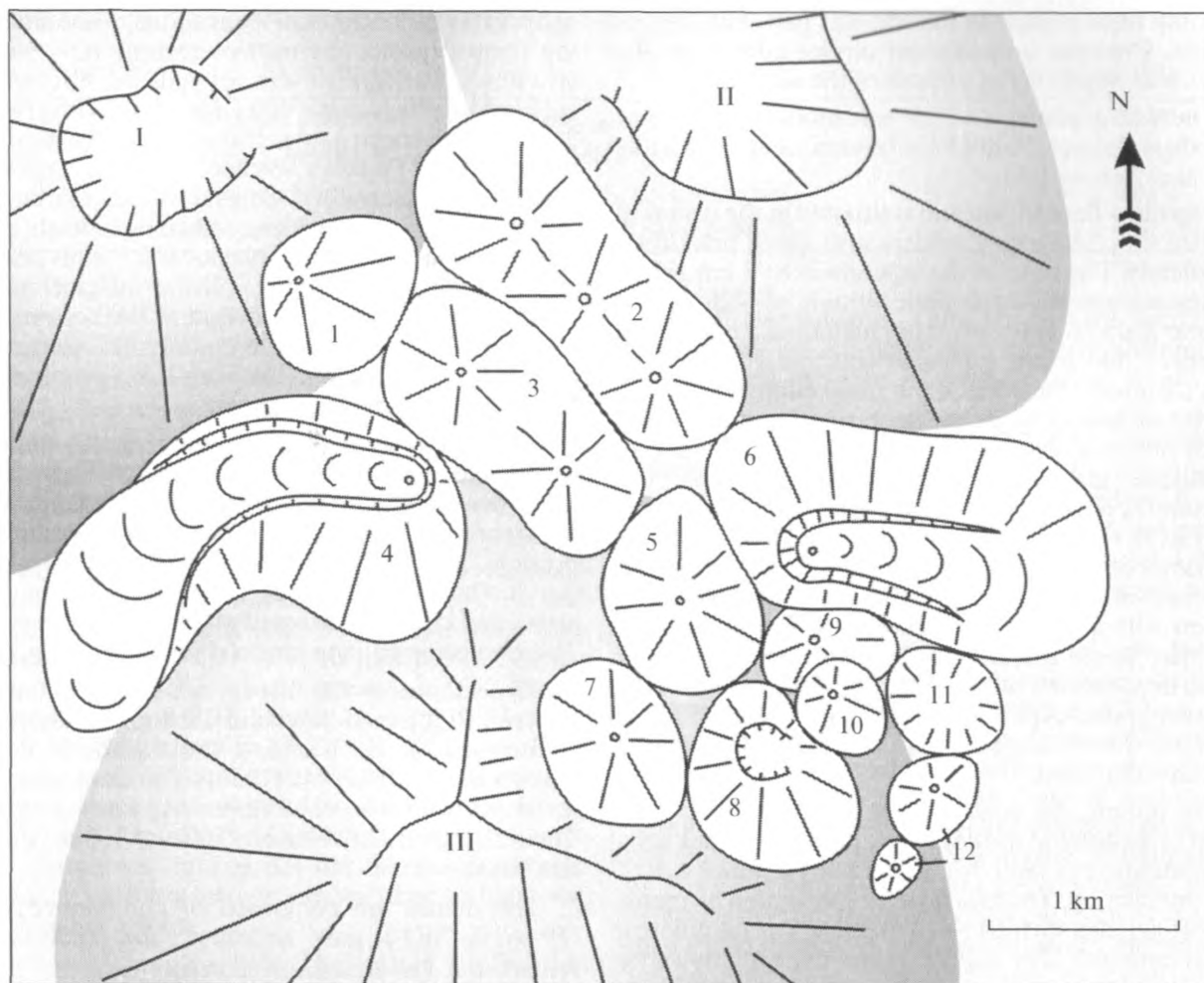
Fig. 6. Set of volcanic domes that are situated in the southeastern part of the Bol'shoi Semyachik massif. I—III volcanoes: Popkova (I), Tsentral'nyi Semyachik (II), Problematichnyi (III). Arabic numerals mark domes (the names are after [Vlodavets, 1958]): (1) "Ivanova Volcano." (2) Kupol "soshchitont" and its series, (3) Kupol "spemzoi" and its series, (4) Korona, (5) Peremychka, (6) Ezh, (7) Yuzhno-Tsentral'nyi, (8) Kupol "s kraterom," (9) Chernyi, (10) Krutoi, (11) Skalistyi, (12) Oval'nye.
