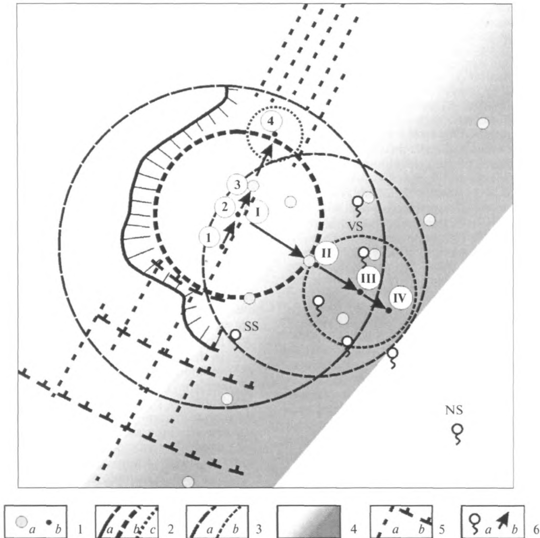
Fig. 8. A map of structural localization for centers of volcanic and hydrothermal activity in the Bol'shoi Semyachik Massif area. (I) centers of volcanic edifices ( a ) and of volcanic fields or reconstructed edifices (A), (2) boundaries of a pre-caldera edifice (Khrebet Bort) ( a ), of the caldera (ft), and of the post-caldera Kulakova Dome rise ( c ), (3) boundary of the area where the post-caldera volcanoes are situated ( b ), (4) zone where the locations of centers of volcanic activity are controlled by regional faults striking northeast, (5) neotectonic faults striking north-northeast ( a ) and west—northwest (ft), (6) sets of thermal springs and steam jets ( a ), directions along which the centers of volcanic activity were migrating ( b ). Numerals in circles (1-4 and I-IV) mark two directions of migration, for detail see main text. For the other notation see Figs. 2 and 3.
