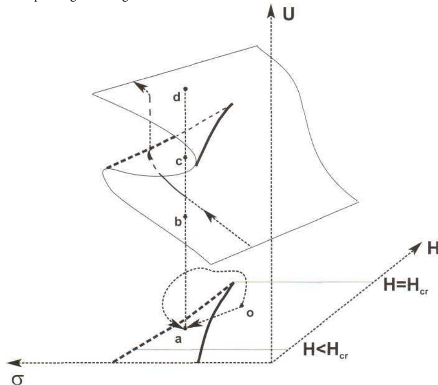
Fig. 9. Magma ascent velocity as a function of governing parameters H and \sigma . The curved plane is an equilibrium surface of the standard catastrophe of two-parameter function with cusp-like singularity (two folds converging onto a cusp). It is drawn as an illustration without calculated figures on the axis. Point 'a' in the \sigma - H plane has three images in the equilibrium surface ('b', 'c' and 'd') showing three feasible states of an eruption. The line with arrows on the equilibrium surface is the trajectory of the image point showing changes due to the conductivity increase at the beginning of an eruption with a sharp increase of the eruption intensity. Two lines connecting points 'O' and 'a' on the \sigma - H plane indicate two possible smooth evolution paths leading to different points ('b' and 'd') on the equilibrium surface.
