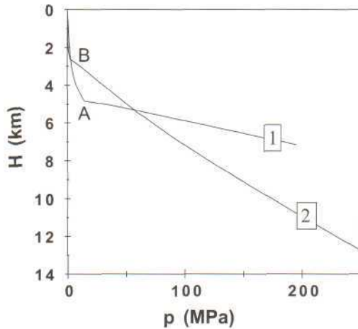
Fig. 6. Pressure variations with height along conduits of volcanoes with different types of magma. (1) Model of the Mount St. Helens 1980 eruption ( H=7.2 km, U \sim 1 m s^{-1} , a=0.0060 MPa^{-1/2} , d_p=0.001 m, c=0.046 ); (2) model of the First Cone at the Northern Breakthrough of the Tolbachik 1975 eruption ( H=25 km, U \sim 0.1 m s^{-1} , a=0.0032 MPa^{-1/2} , d_p=0.01 m, c=0.05 ). Points A and B indicate fragmentation levels for these eruptions.
