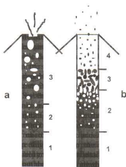
Fig. 2. Possible structures of two-phase flow in a volcanic conduit. (a) The discrete gas separation (DGS) regime: Zone 1, magma without bubbles; Zone 2, single-velocity bubbling flow; Zone 3, DGS (two-velocity bubbling) flow, (b) The dispersion (steady-jet) regime: Zone 1, magma without bubbles; Zone 2, bubbling single velocity flow; Zone 3, partly destroyed foam (PDF, porous, channeled medium); Zone 4, gas-pyroclastic dispersion flow.
