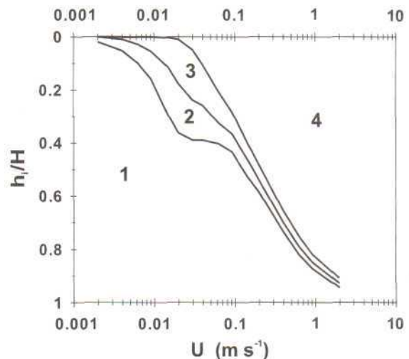
Fig. 7. Map of the relative lengths of the zones with different flow structures, h_i/H versus magma ascent velocity for the dispersion regime. Curves are the boundaries dividing the zones with different flow structures; h_i is the length of zone i . Zone 1 ( i=1 ) is the homogeneous melt; zone 2 is the bubbling flow; zone 3 is the partly destroyed foam (PDF); zone 4 is the dispersion of a two-phase gas-pyroclastic mixture. Parameters used in the calculations: c_0=0.046 ; a=0.0060 MPa^{-1/2} ; \sigma=10^{-4} m^2/Pa s; d_p=0.001 m; p_{ex}=0 .
