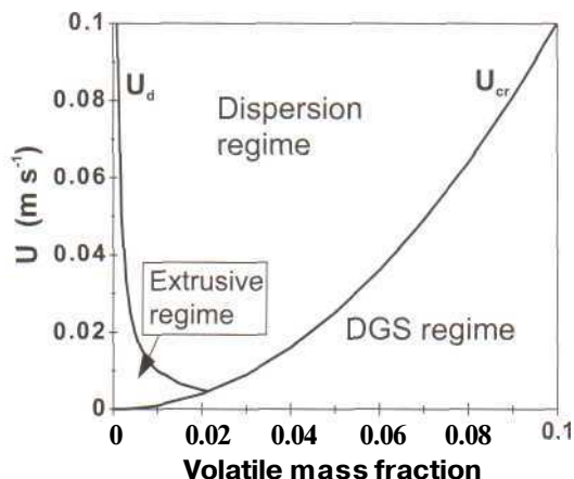
Fig. 4. Map showing eruption regimes on a plot of magma velocity versus volatile (water) content bounded by critical curves. The curve for U_{cr} divides the DGS regime from others, calculated using Eq. 21 with \xi = 5 \times 10^{-3} \text{ s m}^{-1} ; curve U_d divides extrusive and dispersion regimes calculated using Eq. 31 with A = 0.01 .
