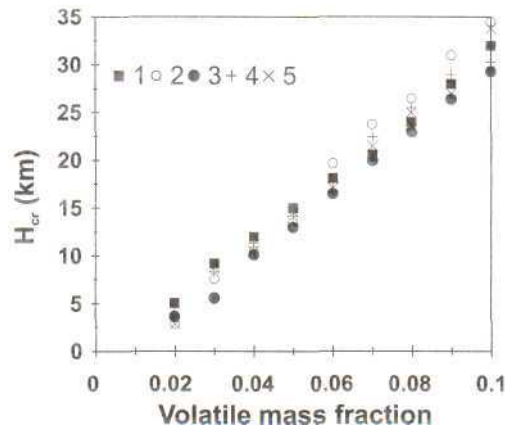
Fig. 20. Value of H_{cr} as a function of volatile (water) content in magma c_0 at p_c = 20 MPa. For other parameters the following values were used: (1) d_p = 0.001 m, \beta = 0.75 , \alpha = 0.0041 MPa ^{-1/2} ; (2) d_p = 0.01 m, \beta = 0.75 , \alpha = 0.0032 MPa ^{-1/2} ; (3) d_p = 0.0001 m, \beta = 0 , \alpha = 0.0041 MPa ^{-1/2} ; (4) d_p = 0.001 m, \beta = 0.3 , \alpha = 0.0064 MPa ^{-1/2} ; (5) d_p = 0.01 m, \beta = 0.75 , \alpha = 0.0041 MPa ^{-1/2} .
