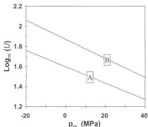
Fig. 19. Amplitude of the magma mass rate jump ( U ) as a function of p_{ex} calculated for a volcano similar to Mount St. Helens ( H=7.2 km). Here U is the change in velocity at the jump. Line A, U=ulu \uparrow (jump upward); line B, U=ulu \downarrow (jump downward).
