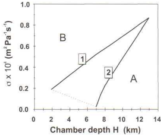
Fig. 10. Projection of the 'cusp' on the plane of the governing parameters (chamber depth and conduit conductivity) or map of catastrophe. Calculated using the same parameters as for Fig. 8. Inside the angle, between lines 1 and 2, every point corresponds to three values of magma velocity: two stable regimes with low and high intensity ('lower' and 'upper' regimes) and one unstable intermediate intensity regime. Region A corresponds to the 'lower' regime only; region B, to the 'upper' (much more intensive) regime.
