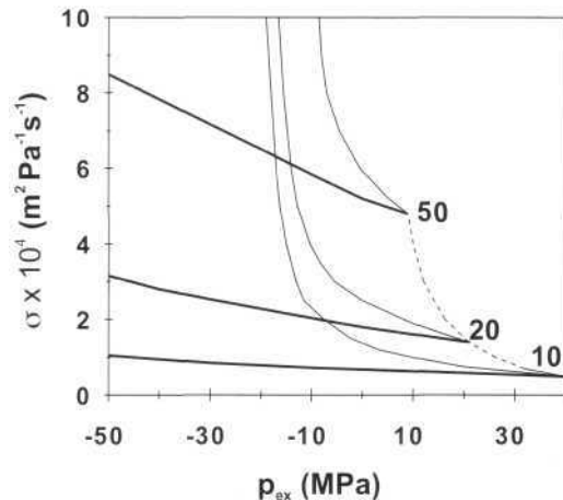
Fig. 23. Maps of catastrophe on the plane p_{ex} - \sigma calculated for a volcano similar to Mount St. Helens and different chamber depths. Bold lines are the lines of the folds describing the jump-like decrease of magma mass rate; thin lines correspond to the folds describing the jump-like increase of magma mass rate. Figures near the cusps (the point where the two lines intersect) are the values of the magma chamber depth in km. The dashed line shows the location of this intersection (cusp) point in p_{ex} - \sigma space.
