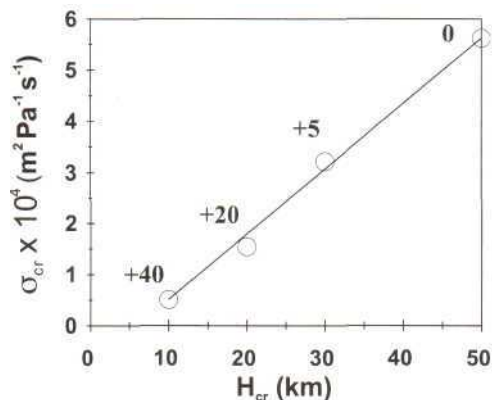
Fig. 13. Change of the position of the cusp point on the coordinate plane H_{cr} - \sigma_{cr} as a result of a p_{ex} change calculated for the parameters corresponding to the Tolbachik eruption (see Fig. 8 for values). The value of p_{ex} in MPa is shown near the points on the graph.
