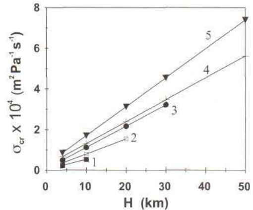
Fig. 14. The dependence \sigma_{cr}(H) at H < H_{cr} calculated at different values of p_{ex} : (1) p_{ex} = 40 \text{ MPa} ( H_{cr} = 10 \text{ km} ), (2) p_{ex} = 20 \text{ MPa} ( H_{cr} = 20 \text{ km} ), (3) p_{ex} = 5 \text{ MPa} ( H_{cr} = 30 \text{ km} ), (4) p_{ex} = 0 ( H_{cr} = 50 \text{ km} ), (5) p_{ex} = -5 \text{ MPa} ( H_{cr} \gg 50 \text{ km} ).
