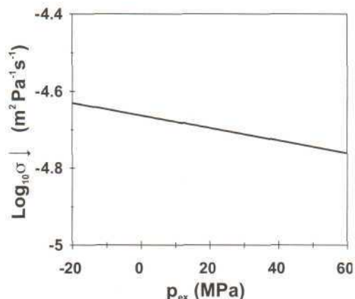
Fig. 17. \text{Log}(\sigma_{\downarrow}) as a function of excess pressure p_{ex} calculated for the Mount St. Helens volcano ( H = 7.2 km).
