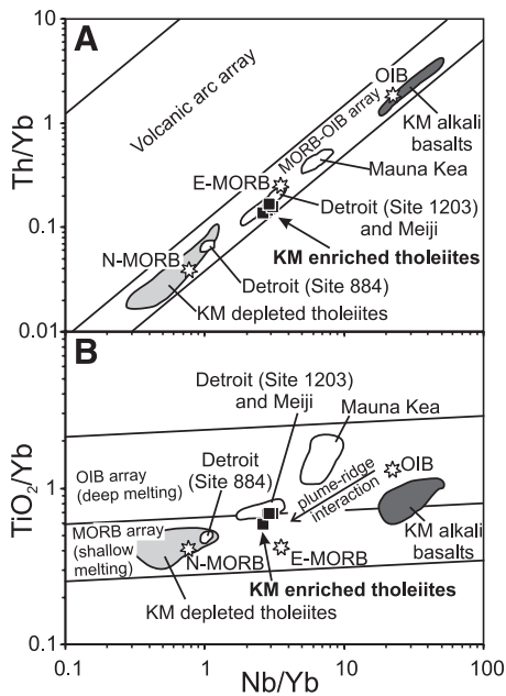
Figure 2. Discrimination diagrams show that volcanic rocks from Kamchatka Mys ophiolites belong to P (plume) type ophiolites after classification of Pearce (2008) and that their immobile incompatible element ratios are similar to shield-stage tholeiites from Detroit (Site 1203) and Meiji Seamounts. Nb, Yb, and Th concentrations are in ppm, TiO 2 in wt%. Compositions of enriched tholeiites from the Kamchatka Mys (KM enriched tholeiites) are from this study; KM depleted tholeiites and alkali basalts are after Saveliev (2003) and Khotin and Shapiro (2006), and references therein. Compositions of average normal mid-oceanic ridge basalt (N-MORB), enriched (E) MORB, oceanic island basalt (OIB) (Sun and McDonough, 1989), Mauna Kea rocks, and Detroit and Meiji shield-stage tholeiites are shown for comparison (data sources listed in Appendix DR1 [see footnote 1]).
