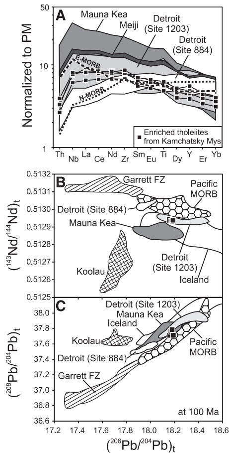
Figure 3. Trace element and isotope compositions of enriched tholeiites from Kamchatka Mys ophiolites. Compositions of typical Pacific mid-oceanic ridge basalt (MORB), depleted MORB from Garrett Fracture Zone (FZ), shield-stage tholeiites from Hawaiian-Emperor Seamount Chain (Mauna Kea, Koolau, Meiji, and Detroit) and Icelandic rocks are shown for comparison (data sources listed in Appendix DR1 [see footnote 1]). Average normal (N) MORB, enriched (E) MORB, and primitive mantle (PM) compositions are after Sun and McDonough (1989). All isotopic compositions are age corrected to 100 m.y. (Table DR2).
